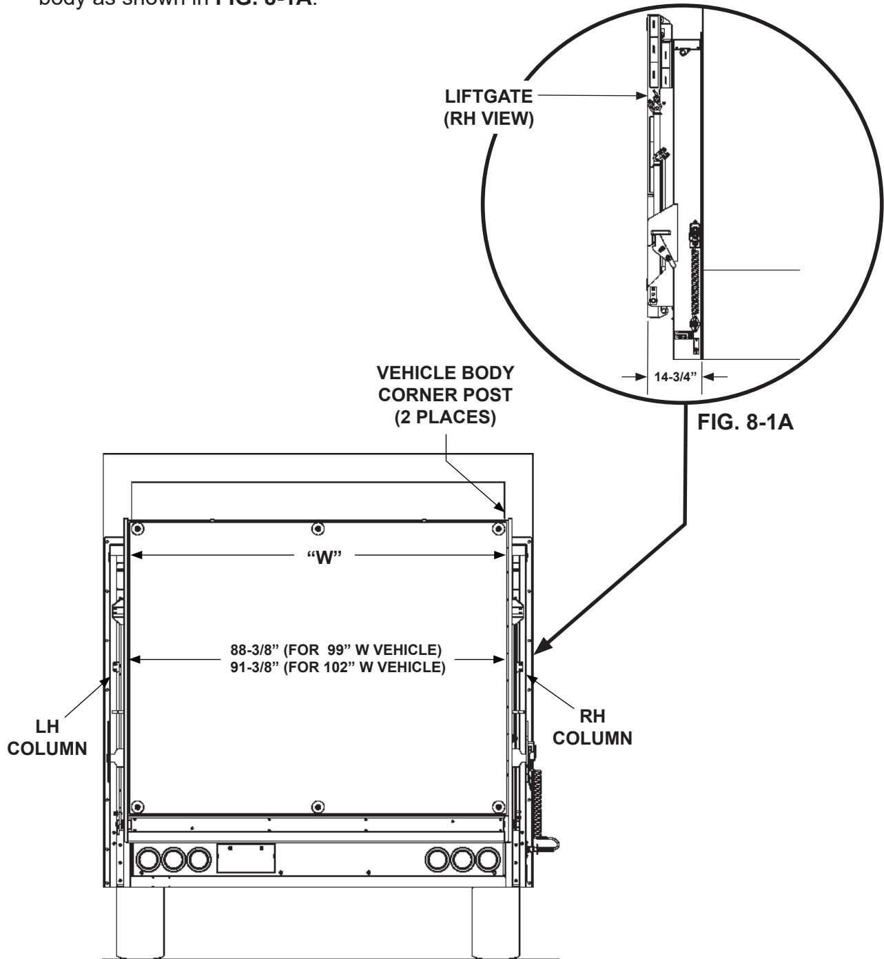
LIFTGATE COLUMNS FITTED TO BODY CORNER POSTS WITH LITTLE OR NO OFFSET FIG. 8-1
