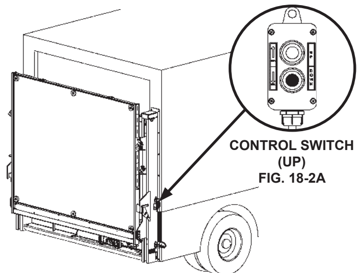
USING CONTROL TO PRESSURIZE HYDRAULIC SYSTEM FIG. 18-2
